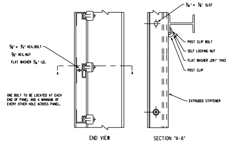
TYPICAL MOUNTING FOR EXTRUSHEET SIGN PANEL
